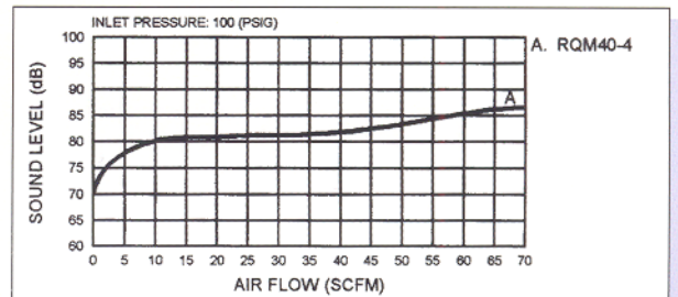
RQM40-4 dB Rating vs. Air Flow
