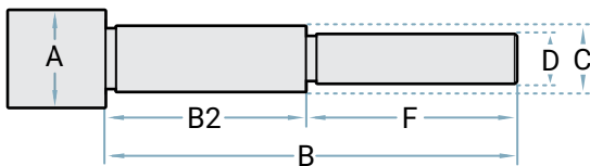
Fixed Journaled Drive End BLN, BLB
