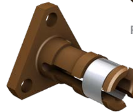
Triangle Constant Force Anti-Backlash Nut p 15
