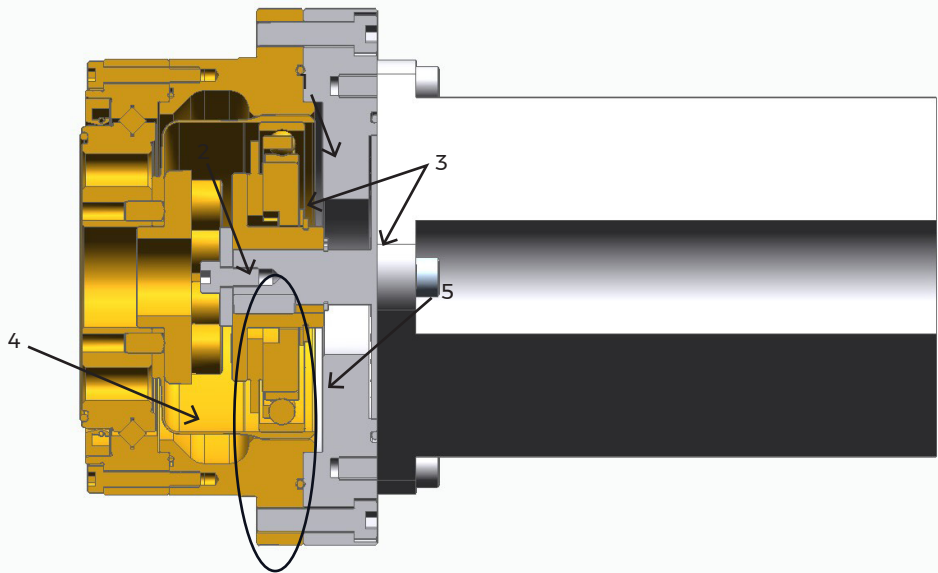
Figure 5. Gearhead to Motor Installation: Cup Style
